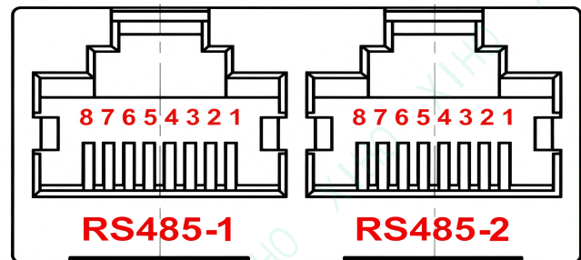
RJ45 Socket
